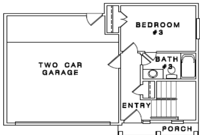
FRONT FLOOR PLAN
