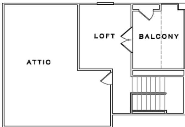
BALCONY FLOOR PLAN
